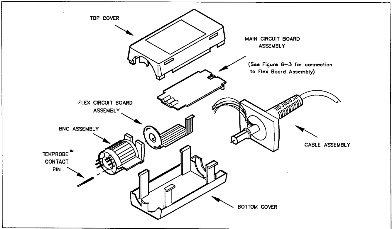
Figure 6-2. Assembly replacement.
