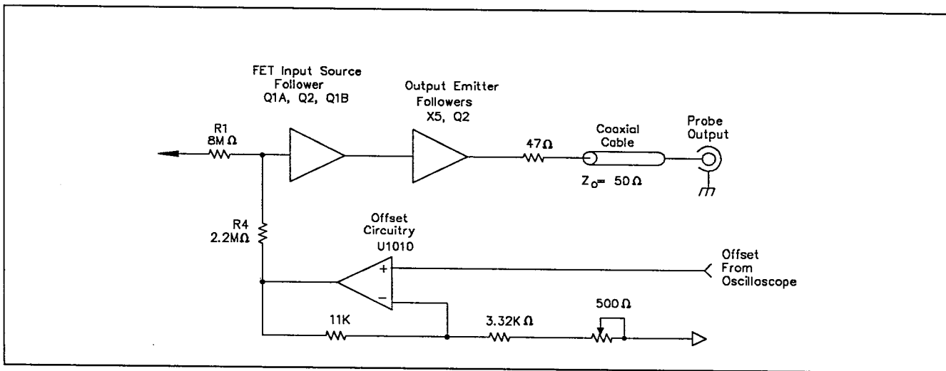
Figure 5-1. Functional block diagram.
