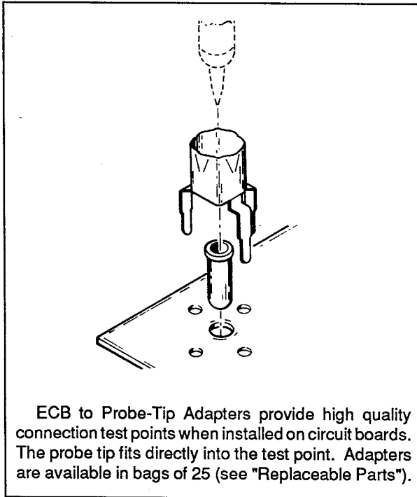
Figure 2-4. Inductance reducing connectors.
