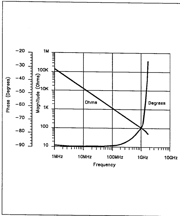
Figure 1-1. Typical Input Impedance vs frequency.
