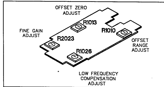
Figure 4-1. Compensation box adjustment locations.
