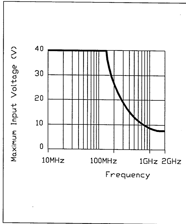
Figure 1-2. Operating voltage derating.
