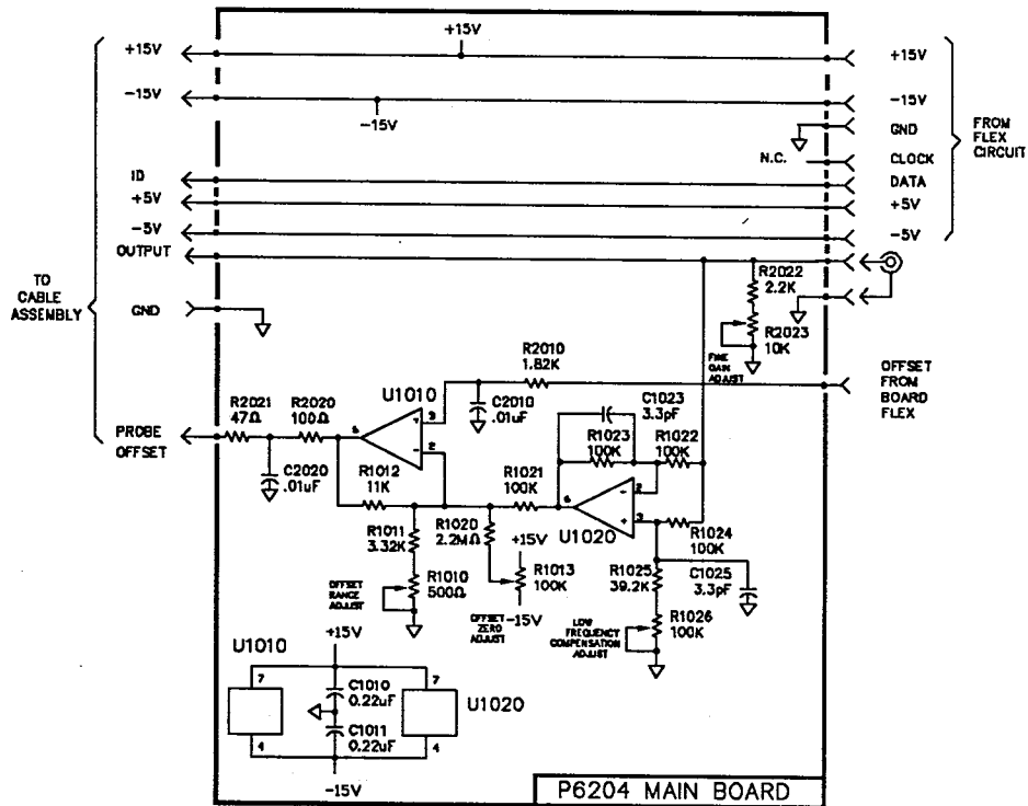
Figure 7-1. The P6204 Main board schematic
