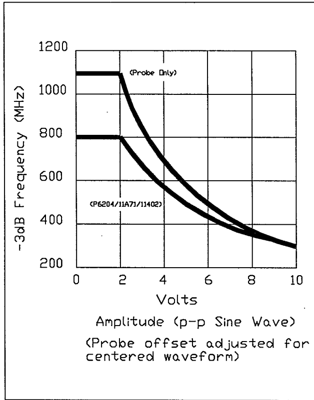
Figure 2-2. Typical -3dB frequency versus amplitude.
