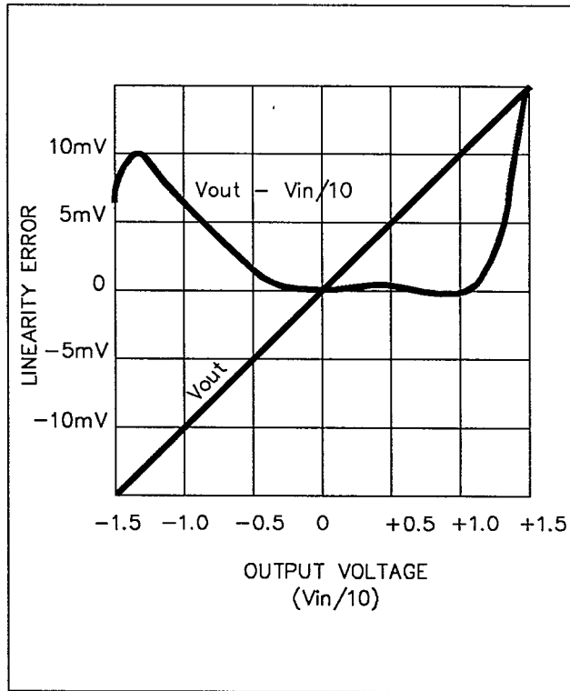
Figure 1-3. Typical Linearity Curve.
